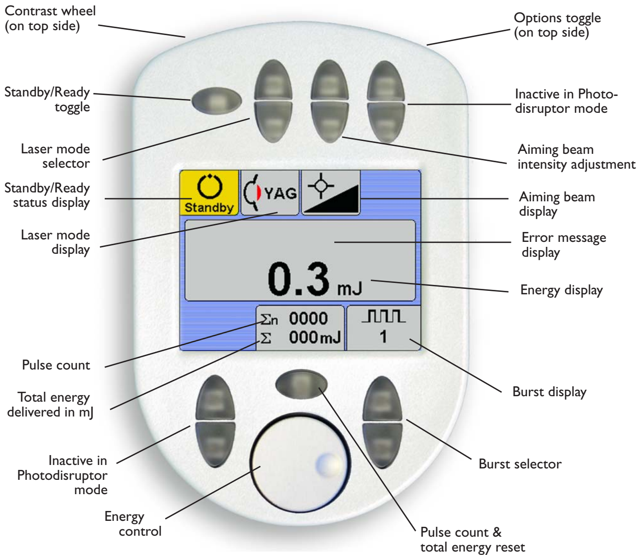
Remote control (Photodisruptor-1064 nm screen shown)
